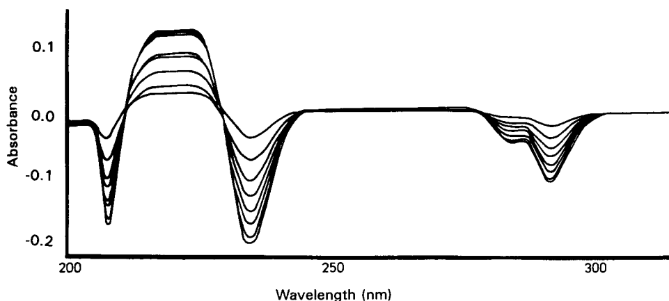
FIG. 2. UV differential spectra of complexes between p -Cl- m -cresol (0.25 mM) and HP- \beta -CyD (0.3–5.0 mM) in phosphate buffer pH 7.4.
