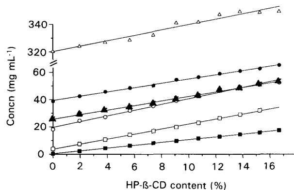
FIG. 1. Effect of HP- \beta -CD on solubility of preservatives in phosphate buffer pH 7.4. \Delta bronopol, \bullet benzylalcohol, \blacktriangle 2-phenoxyethanol, \circ chlorhexidine diacetate, \square p -Cl- m -cresol, \blacksquare p -hydroxybenzoate.
