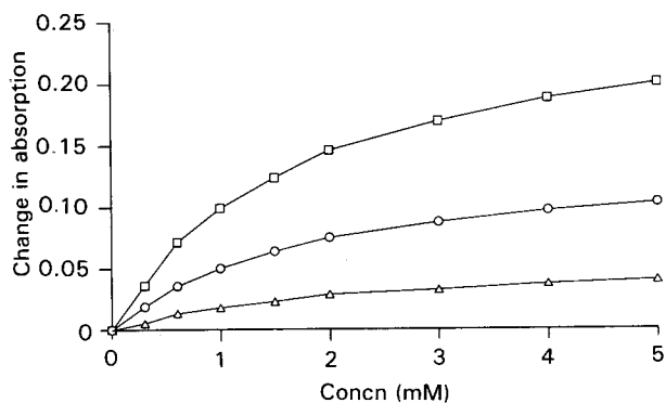
FIG. 3. Absorption shift of p -Cl- m -cresol (0.25 mM) in the presence of HP- \beta -CyD (0.3–5.0 mM), measured at 234 \square , 286 \Delta , 292 \circ nm.
